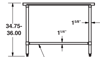
ADJUSTABLE BRACING AT REAR AND SIDES
