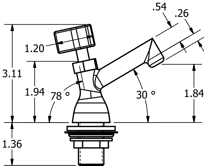
BKF-DWF FRONT VIEW Scale = 1:2
