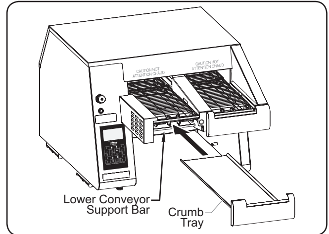
Installing a Crumb Tray (ITQ-1750-2C shown)
