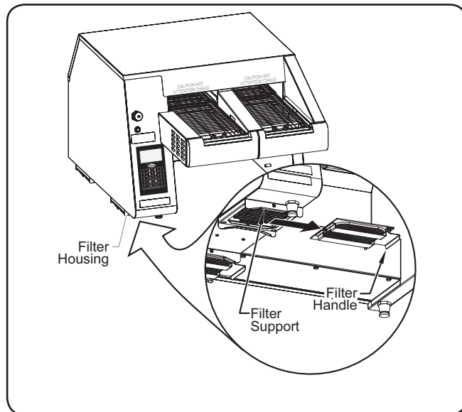
Removing/Installing the Filters
