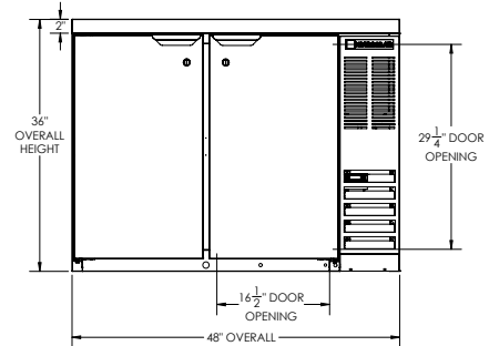
ELEVATION VIEW
